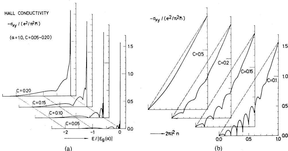
Fig. 6. Examples of \sigma_{XY} of the ground Landau level in case of scatterers with a Gaussian potential. c=2\pi l^2 N_i . See also Figs. 6~11. (a) \sigma_{XY} as a function of the energy. (b) \sigma_{XY} as a function of total number of electrons.
